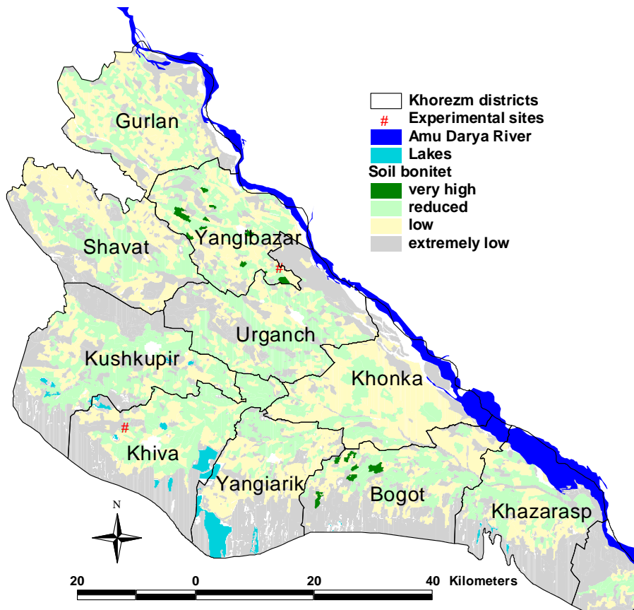
Figure 1. Soil validity for agricultural crops
